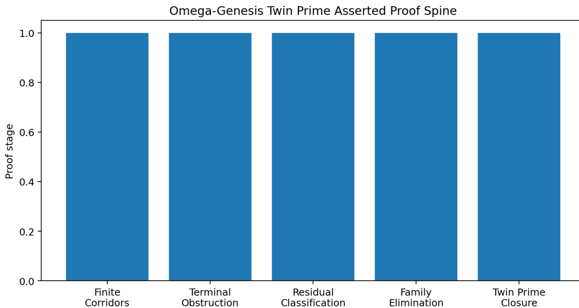
Figure 3. Asserted proof spine.
