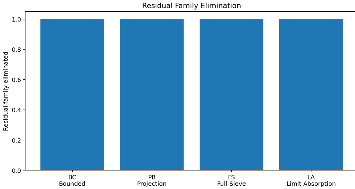
Figure 2. Residual family elimination.
