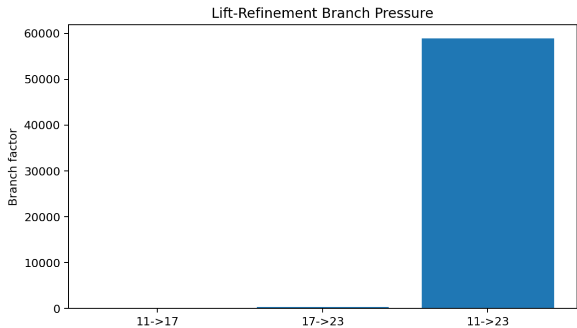
Figure 1. Lift-refinement branch pressure.
